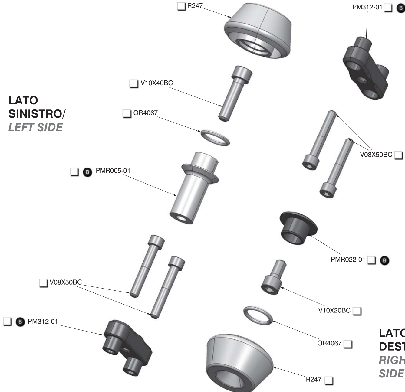
PM312-SX (Para carena lato SX) B (LH Fairing guard)
