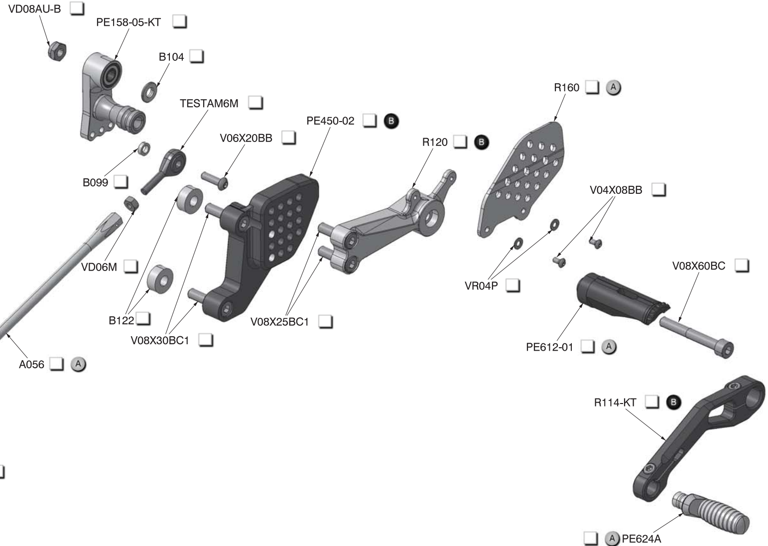
PE450-SX (Complete LH rear set control kit) B
